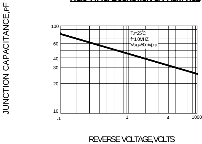
FIG.5-TYPICAL JUNCTION CAPACITANCE
